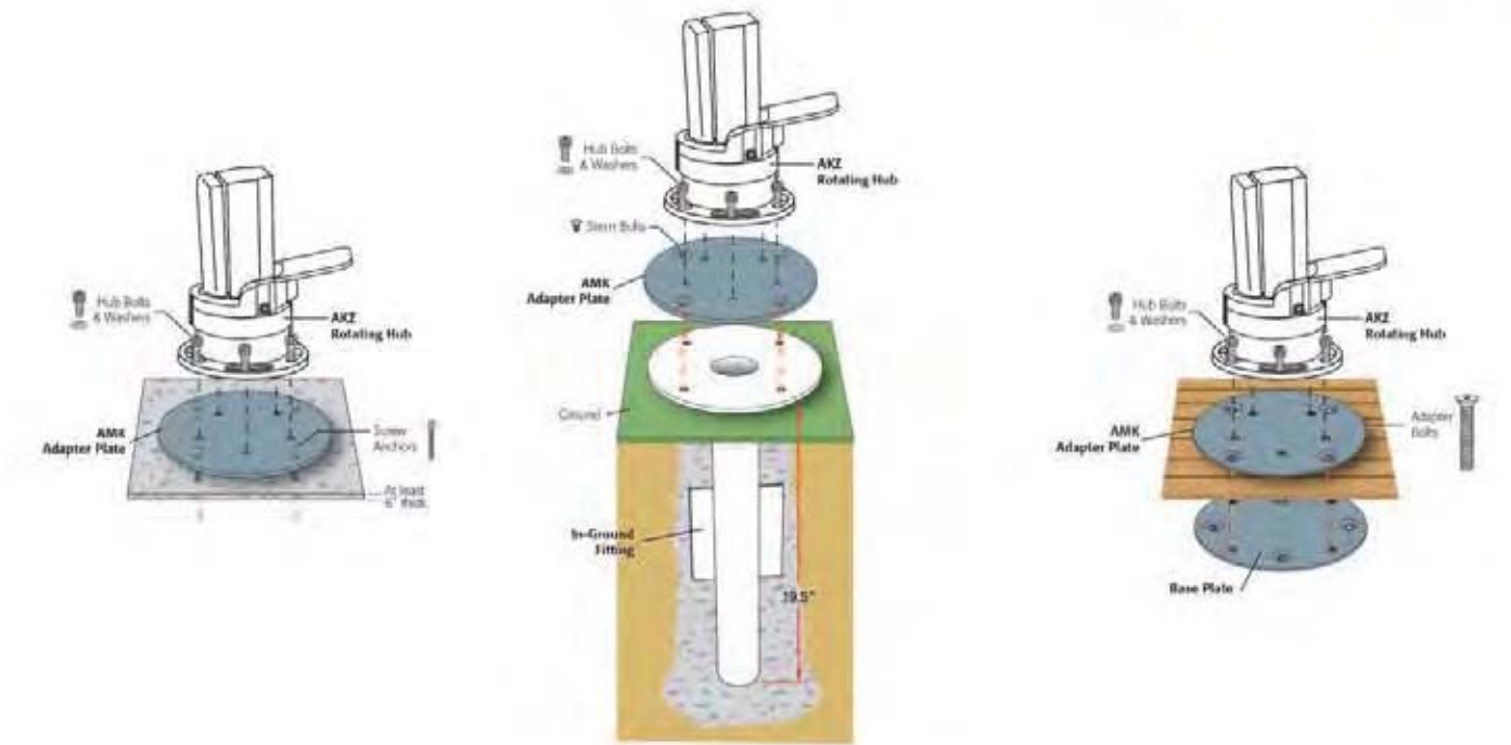
Concrete Mount
