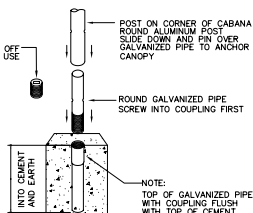
IN-GROUND MOUNTING
