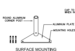
SURFACE MOUNTING
